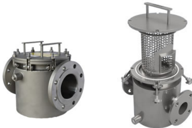
Pipeline Magnet - Closed and Open (showing strainer)
